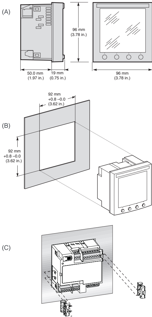
A. Meter dimensions, showing depth behind panel, and display bezel side and front dimensions.
